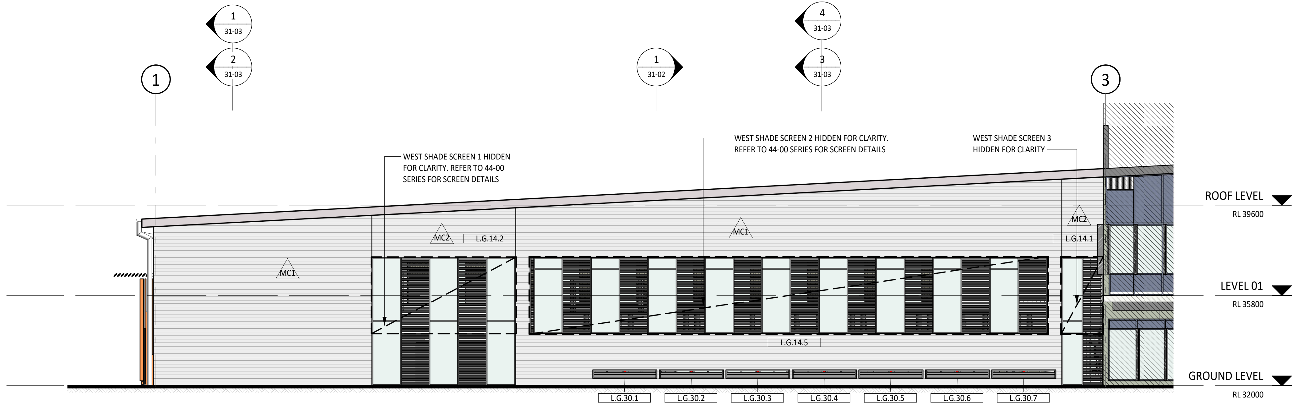
1 BUILDING ELEVATION - WEST - 1 21-00 1 : 100
